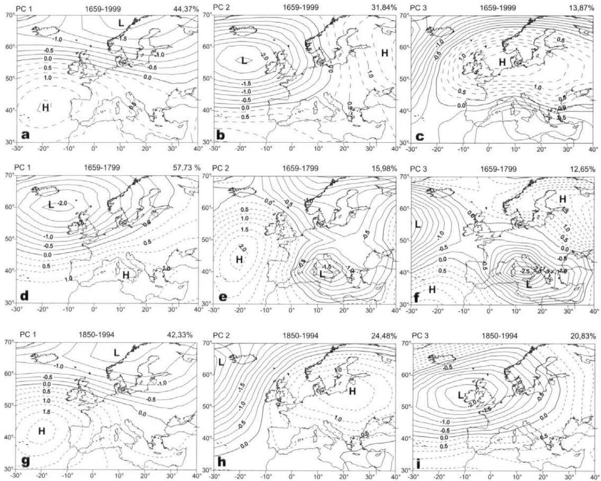
Fig. 8: SLP patterns of the first three PCs of monthly mean SLP grids during winter months: a–c) for all SLP grids between 1659 and 1999; d–f) for the winter months with flood events at the rivers Main, Rhine, Elbe or Weser between 1659 and 1799 (pre-instrumental period); g–i) like d–f, but for 1850–1994 (instrumental period)
